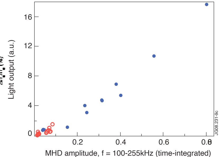
JET (Kiptily NF 2009 Fig. 5)
